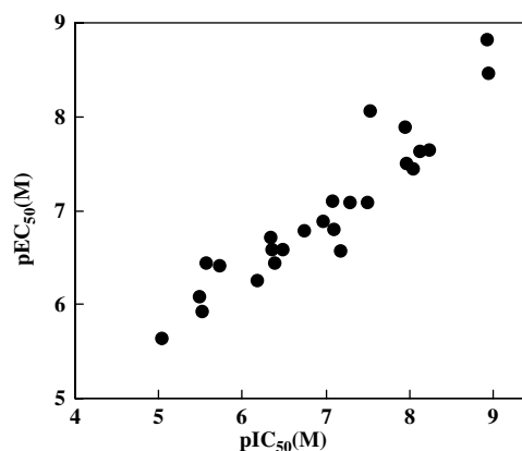
Figure 6. Relationship between the binding ( \text{pIC}_{50} ) of ecdysone agonists to Sf-9 cells and their molting hormonal activity ( \text{pEC}_{50} ) measured in the cultured integument of C. suppressalis .
