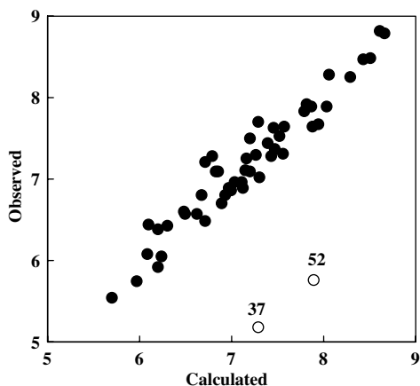
Figure 5. Graphical representation of observed \text{pIC}_{50} values versus \text{pIC}_{50} values calculated with Eq. 2 for 50 compounds (closed circles). Open circles are omitted compounds (37 and 52) in the correlation analysis.
